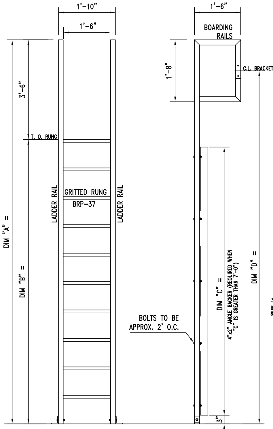
FRP LADDER W/ BOARDING RAILS
