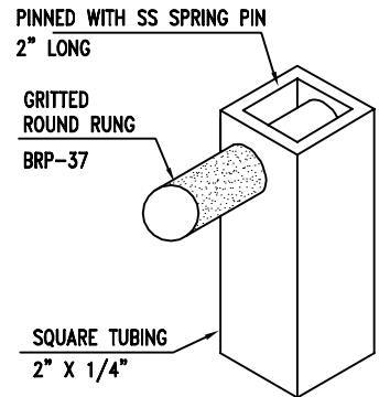
FRP RUNG DETAIL
